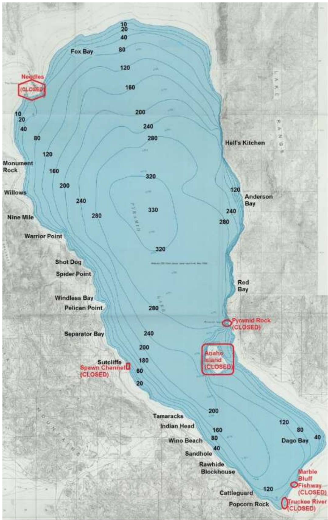
Harris, E.E., 1970, Reconnaissance bathymetry of Pyramid Lake, Washoe County, Nevada: U.S. Geological Survey Hydrologic Investigations Atlas HA-379
